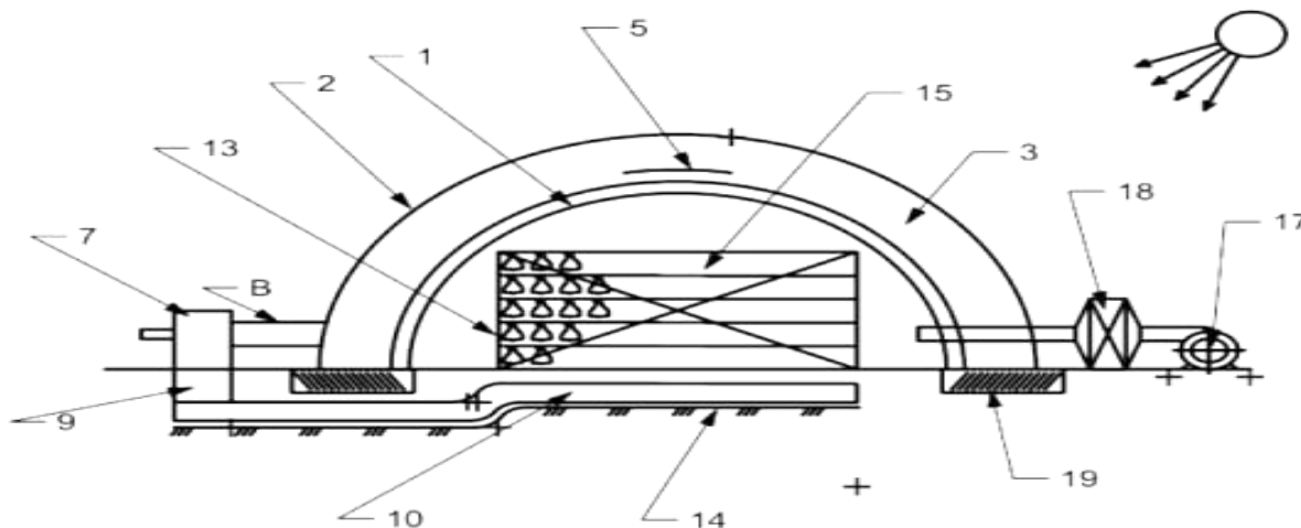
Fig. 3.2. Cross section of pneumatic dryer
