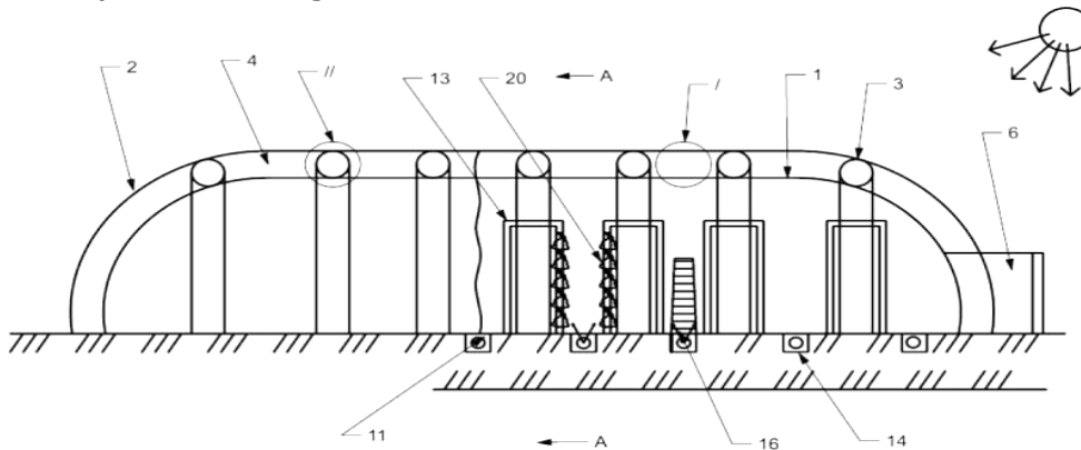
Fig.3.1. Double-layer pneumatic structure as a solar-radiation drying plant for drying grapes
