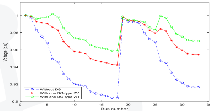
Fig. 4. Impact of two DG units on the voltage profile.
